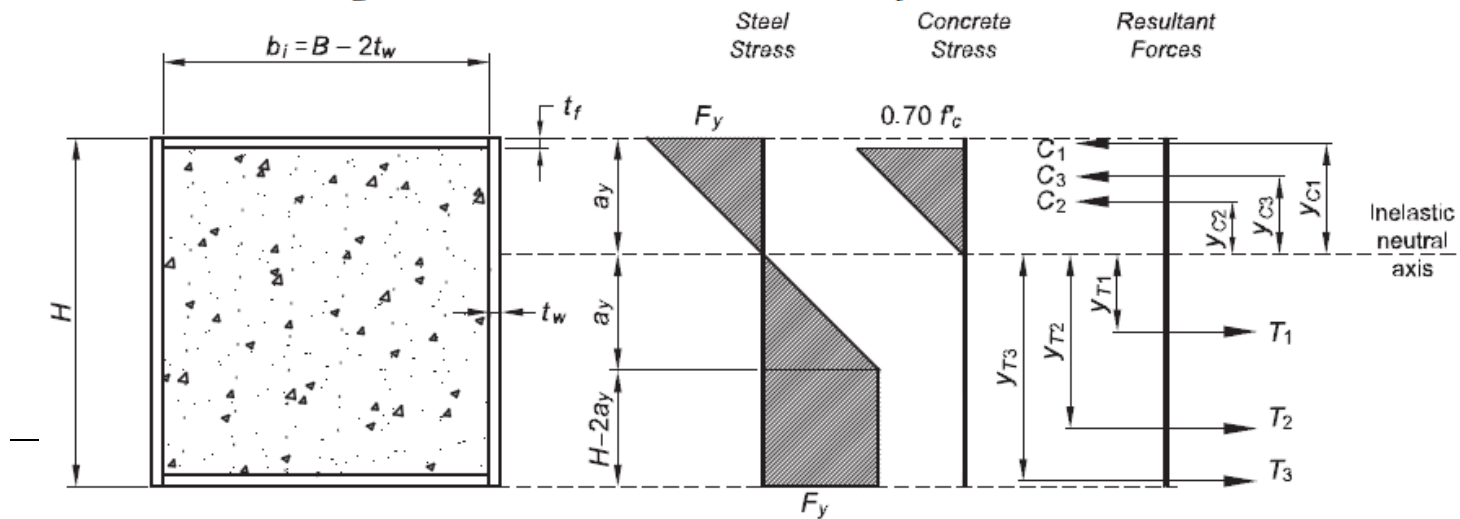
Figure I.7-2. Plastic moment stress blocks and force distribution.
