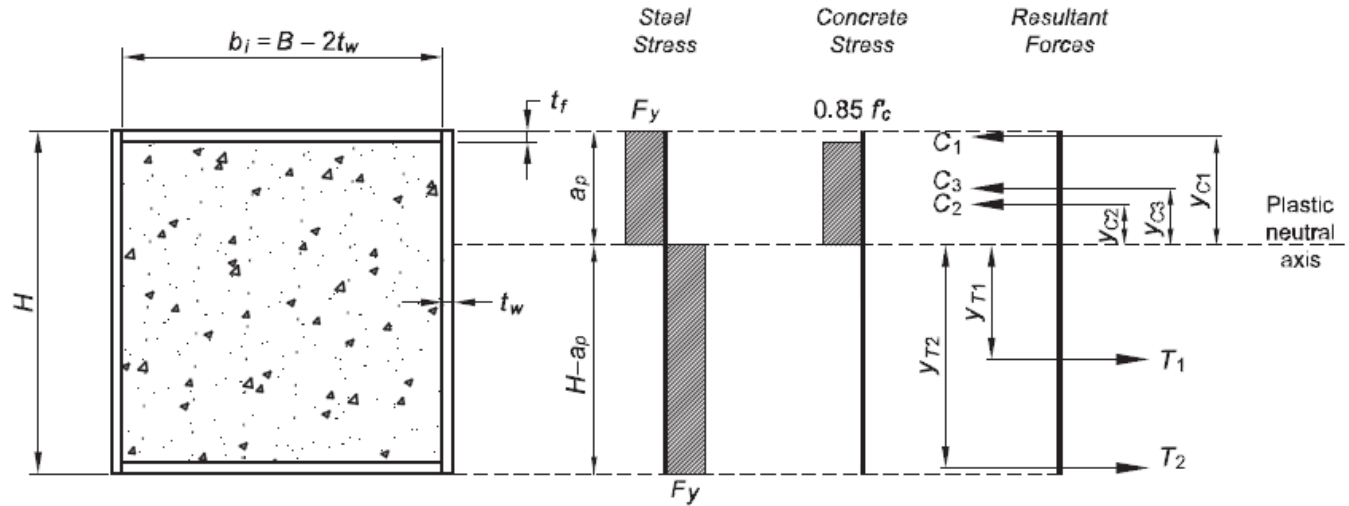
Figure I.7-2. Plastic moment stress blocks and force distribution.
